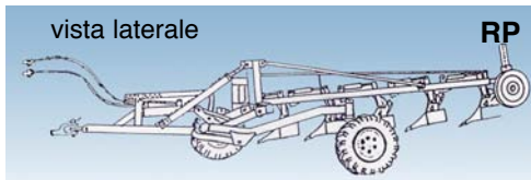
Carrello con aratro a 5 vomeri Trailer with plough and 5 shares
